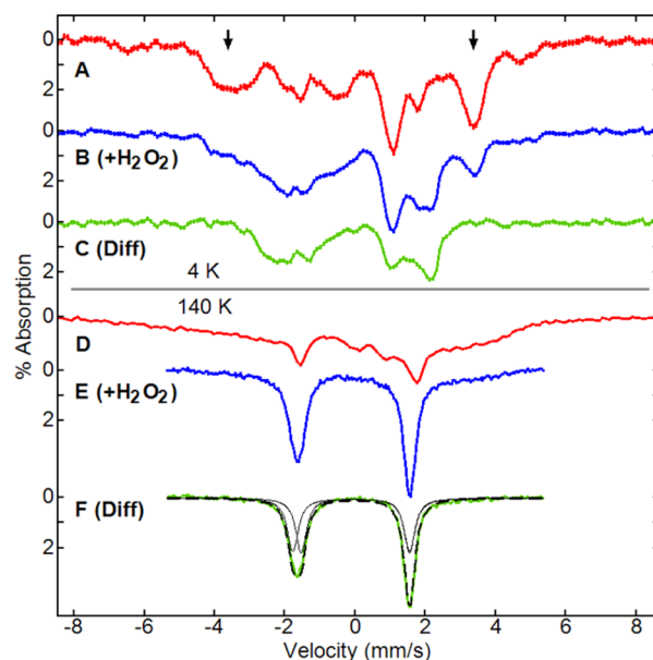
Figure 5. Mössbauer spectra with a parallel field of 45 mT at 4.2 K (A–C) and 140 K (D–F) of (A, D) 1a at pH 11.8 (0.1 M phosphate), 50% glycerol; (B, E) 1a + 1 equiv of \text{H}_2\text{O}_2 , added at -20 \text{ }^\circ\text{C} ; and (C, F) 3a , \text{Fe}^{\text{III}}\text{Fe}^{\text{IV}} . The spectra of \text{Fe}^{\text{III}}\text{Fe}^{\text{IV}} are subtractions of 45% of the spectra of 1a from the spectra with 1a + \text{H}_2\text{O}_2 . At 140 K (F), the simulation (dashed line) is for two quadrupole doublets with equal area (solid black lines) with parameters given in the text.
