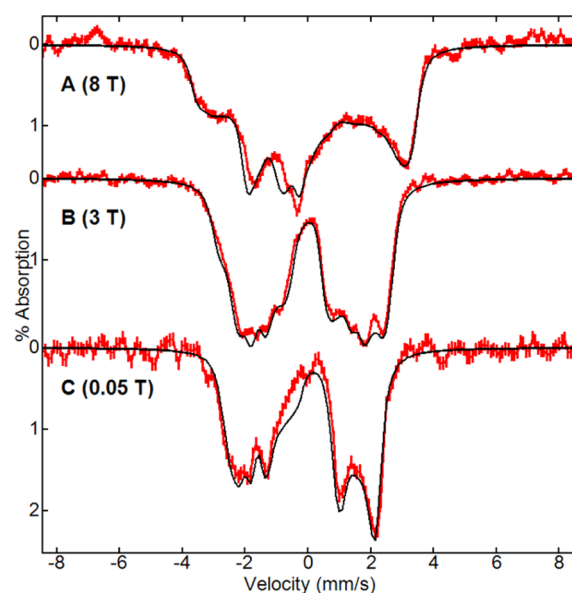
Figure 6. Mössbauer spectra (red lines) of 3a at pH 11.8, 50% glycerol, 1 equiv of \text{H}_2\text{O}_2 recorded at 4.2 K with an applied field of 8 T (A), 3 T (B), and 0.05 T (C). The spectra are after subtraction of 45% of the area the corresponding spectra of 1a . Simulations (black lines) are for \text{Fe}^{\text{III}} and \text{Fe}^{\text{IV}} sites: J = -30 cm ^{-1} , S_3 = 1.5 , D_3 = 3.2 cm ^{-1} , E/D_3 = 0.18 , A_3 = (-45, -120, 55) MHz, S_4 = 1 , D_4 = 21 cm ^{-1} , E/D_4 = 0.13 , A_4 = (-112, -151, 110) MHz for the values of \delta and \Delta E_Q given in the text.
