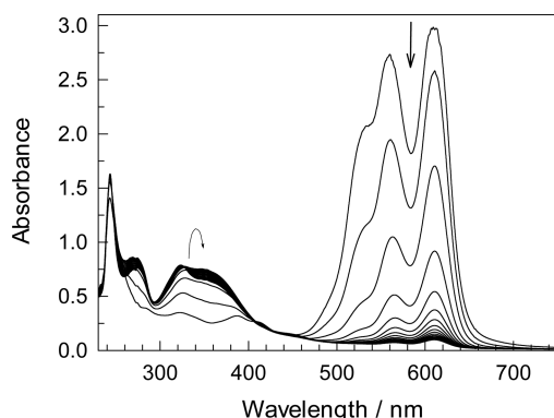
Figure 12. Spectral changes that accompany 1a -catalyzed oxidation of PNC by \text{O}_2 in the reverse micelles. Conditions: [PNC] 4.5 \times 10^{-5} M, [1a] 5.0 \times 10^{-6} M, w_0 10, pH 10, spectra shown with 10 min intervals.
