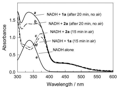
Figure 9. UV-vis spectra of \text{NADH} in the presence of 1a or 2a (1.5 mL methanol was added to 1.5 mL reaction mixture to quench the reaction). Conditions: w_0 7, pH 12, [\text{NADH}] 2.1 \times 10^{-4} M, [\text{total iron}] = 2.0 \times 10^{-4} M. (a, b) spectra of \text{NADH} reacted with 1a or 2a in the absence of \text{O}_2 ; c, d) spectra of \text{NADH} reacted with 1a or 2a after exposure to air for 15 min; e) spectrum of \text{NADH} alone.
