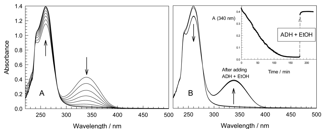
Figure 8. (A) Spectral changes that accompany 1a -catalyzed oxidation of NADH into \text{NAD}^+ by \text{O}_2 and (B) regeneration of NADH by ADH/EtOH. Time interval between spectra shown in A is 20 min (scans were made every 30 s). ADH (from Saccharomyces cerevisiae , 0.7 mg, 210 units in 50 \mu\text{L} water) and 10 \mu\text{L} of EtOH were added to the reaction mixture after 3 h followed by vigorous shaking. Inset in B illustrates the time scale of TAML-catalyzed oxidation and the enzyme-catalyzed regeneration of NADH. Conditions: 0.1 M AOT, 0.01 M carbonate (pH 10), w_0 7; [ 1a ] 2.46 \times 10^{-6} M, [ \text{NADH} ] 9.9 \times 10^{-5} M.
