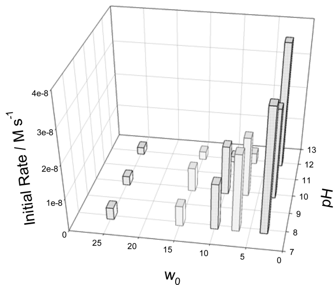
Figure 10. Initial rates of \text{NADH} oxidation catalyzed by 1a in reverse micelles. Conditions: [\text{1a}] 2.5 \times 10^{-6} M, [\text{NADH}] 5.1 \times 10^{-5} M, the flash frequency is 30 s. See text for explanations.
