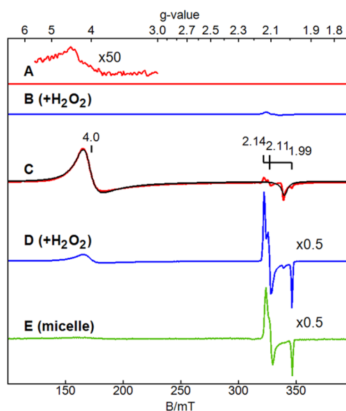
Figure 3. EPR spectra ( \nu = 9.651 GHz, T = 15 K) of 1a at pH 12 under different conditions. A: 1a ; B: 1a + 1 equiv of H 2 O 2 ; C: 1a in 50% glycerol; D: 1a + 1 equiv of H 2 O 2 in 50% glycerol; E: 1a in reverse micelles ( w_0 10, pH 12). The spectral intensities are displayed for equal concentrations of 1a , with additional scale factors as displayed. The black line on C is a simulation for S = 3/2 , D = +2.5 cm -1 , E/D = 0 , g = 2.045, 2.05, 2.03 , \sigma_g = 0.15, 0.15, 0.02 ). The species percentages are stated in the text. A small variable amount ( \sim 2\% ) of 3a is generated in air without H 2 O 2 , which is presumed to be reaction of 1a with low levels of dioxygen.
