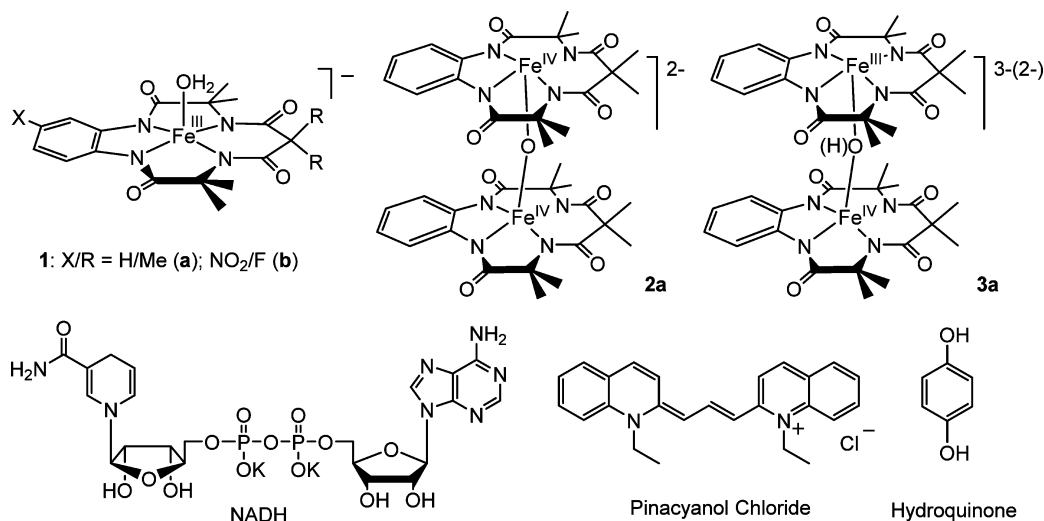
Chart 1. Compounds Used in This Study Including the Catalysts 1a and 1b, the Known Homovalent \mu -Oxo-Bridged Iron(IV) Dimer 2a and Heterovalent \mu -Oxo(hydroxo)-Bridged Iron(IV/III) Dimer 3a Characterized in This Work, and the Substrates \beta -Nicotinamide Adenine Dinucleotide, Reduced Dipotassium Salt (NADH), Pinacyanol Chloride (PNC), and Hydroquinone (HQ)
